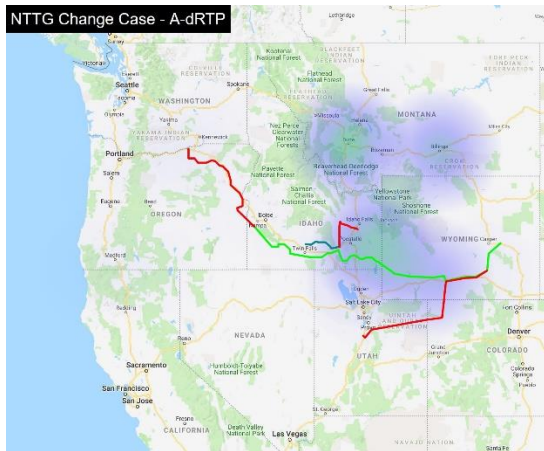
Figure 71 – Heavy Summer Case with dRTP configuration
